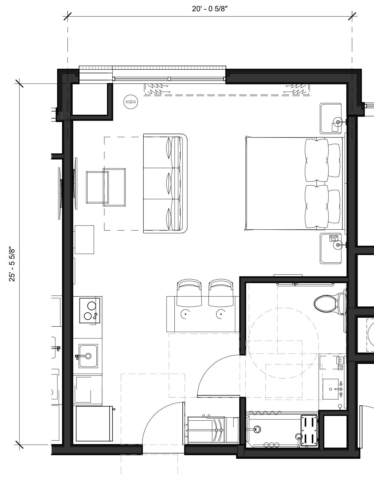
4 ENLARGED ACC KING STUDIO SUITE 1/4" = 1'-0"
