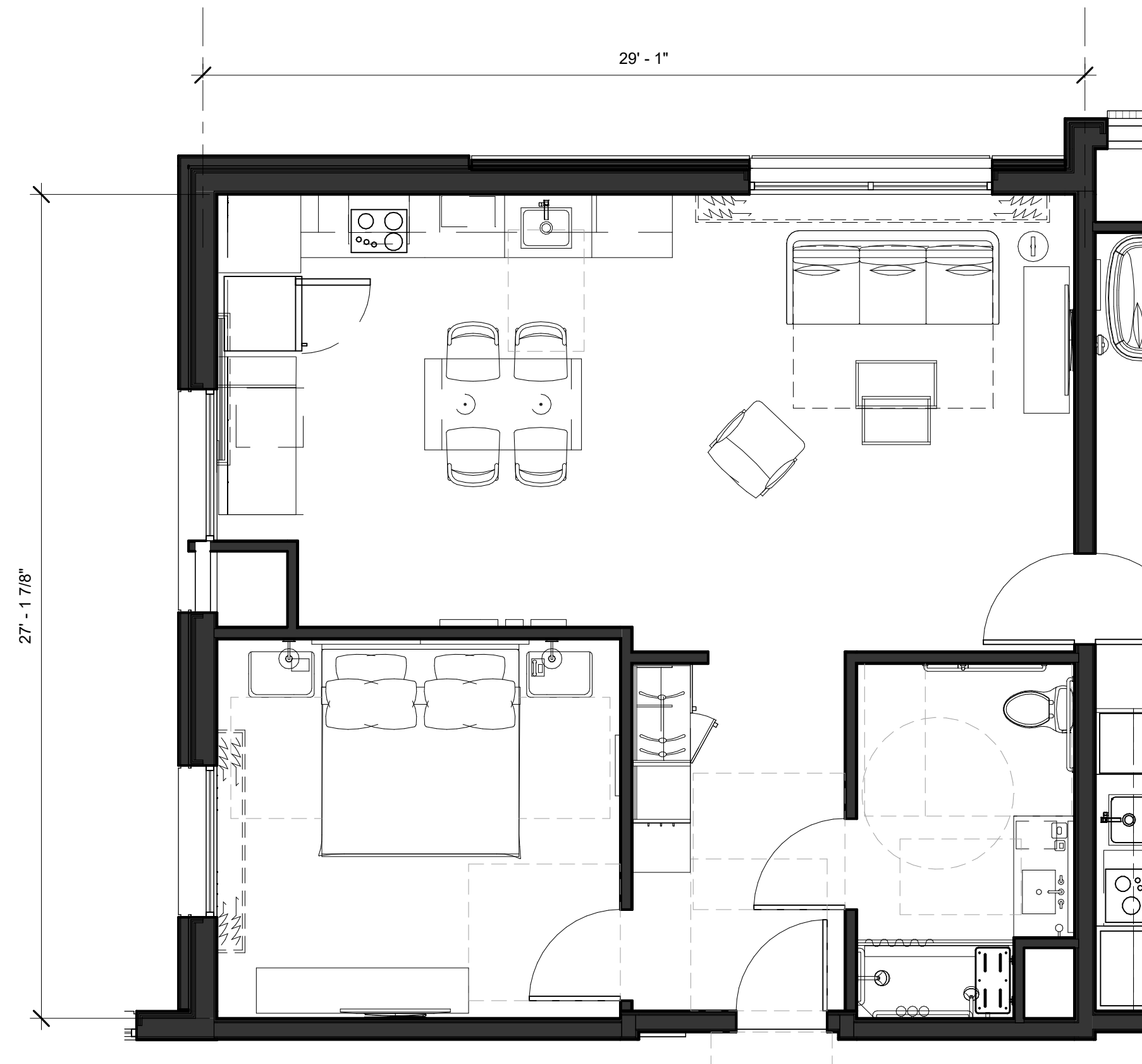
6 ENLARGED ACC KING ONE BEDROOM SUITE 1/4" = 1'-0"
