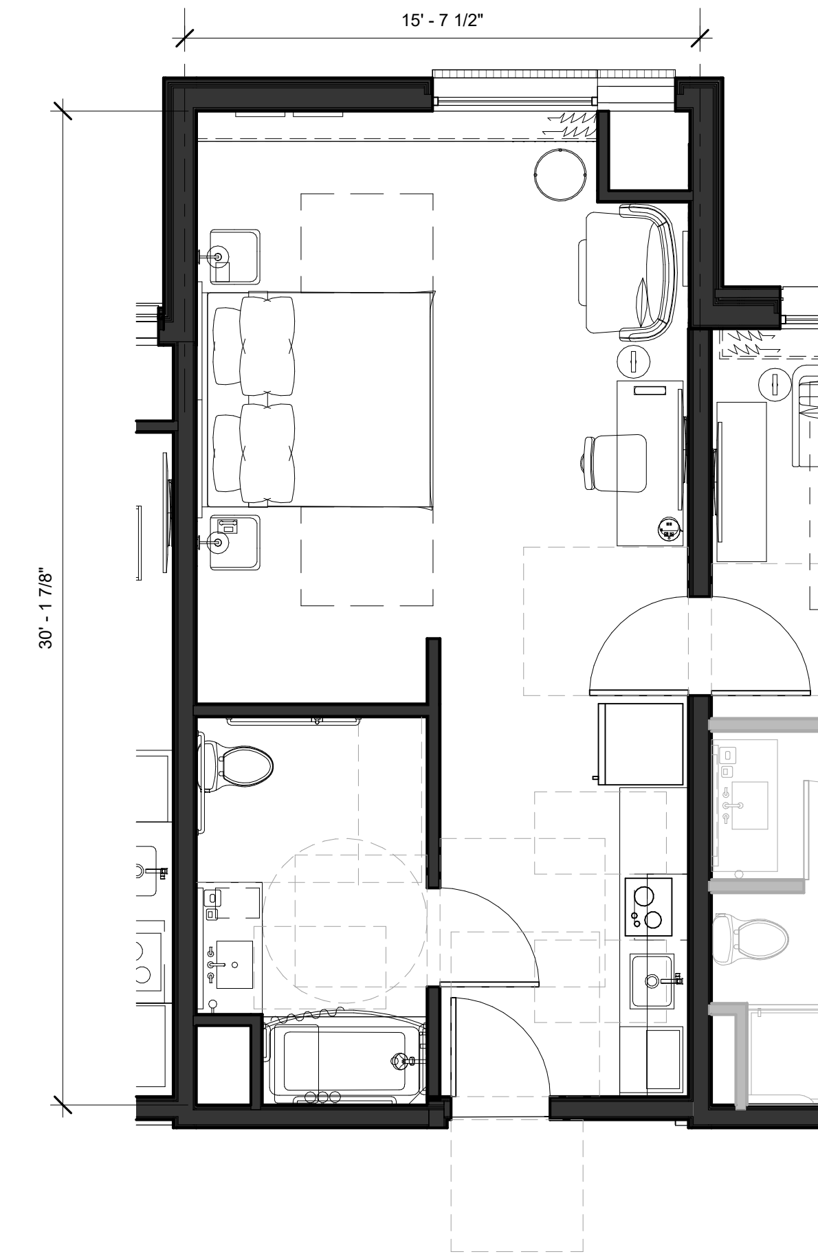
2 ENLARGED ACC EFFICIENCY SUITE 1/4" = 1'-0"
