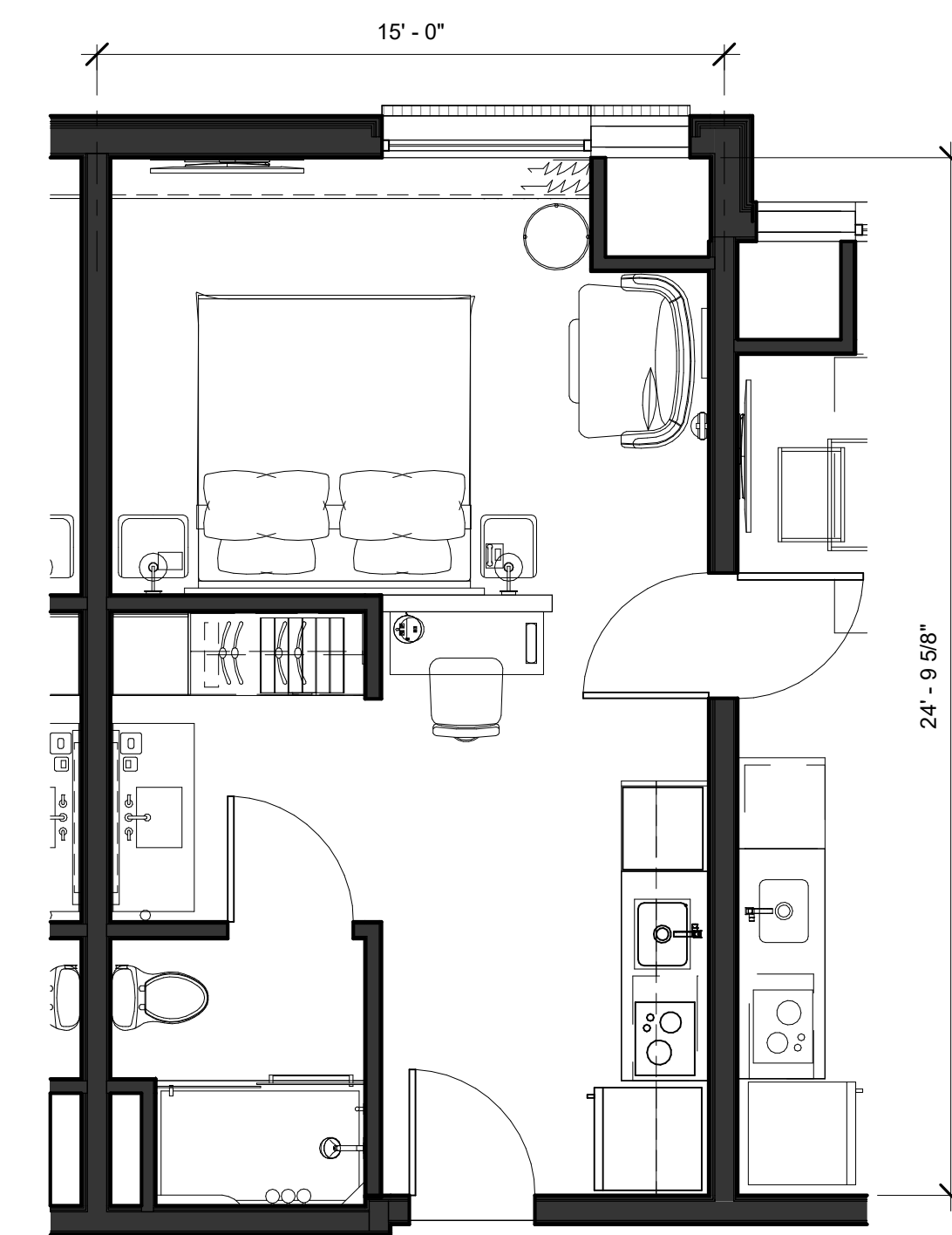
1 ENLARGED EFFICIENCY SUITE 1/4" = 1'-0"
